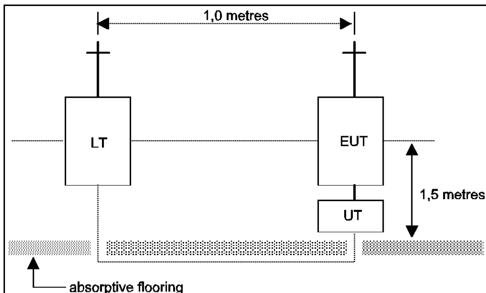
Figure 23: Testing arrangement
