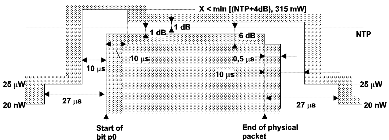
Figure 33a: Power-time template for GFSK modulated packet
