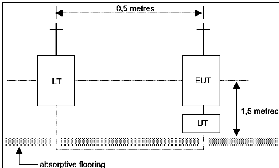
Figure 22: Testing arrangement
