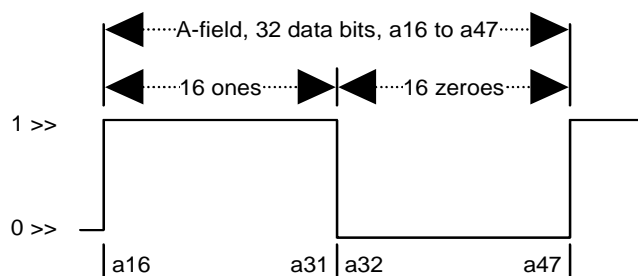
Figure 34: Test packet structure for case 2, A-field
