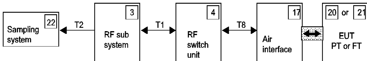
Figure 18: Test setup 1
